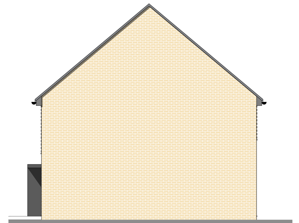
Side 2 Elevation 1:100
