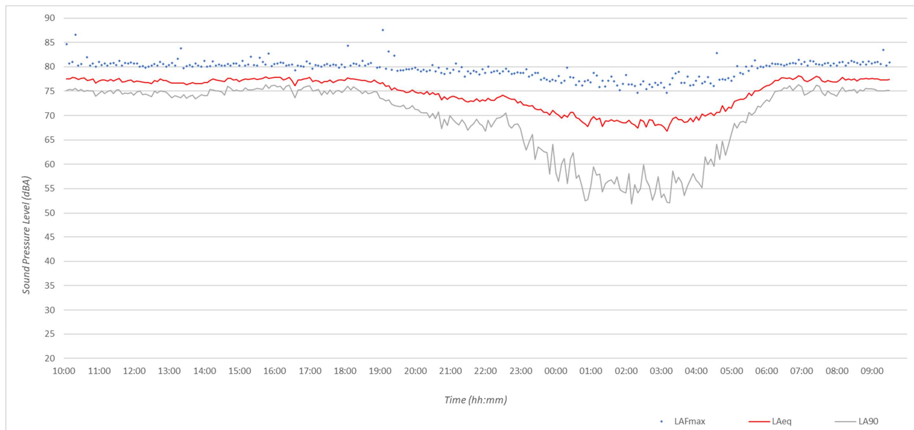
Environmental Noise Measurement M1 Time History: 24 – 25 th September 2024
