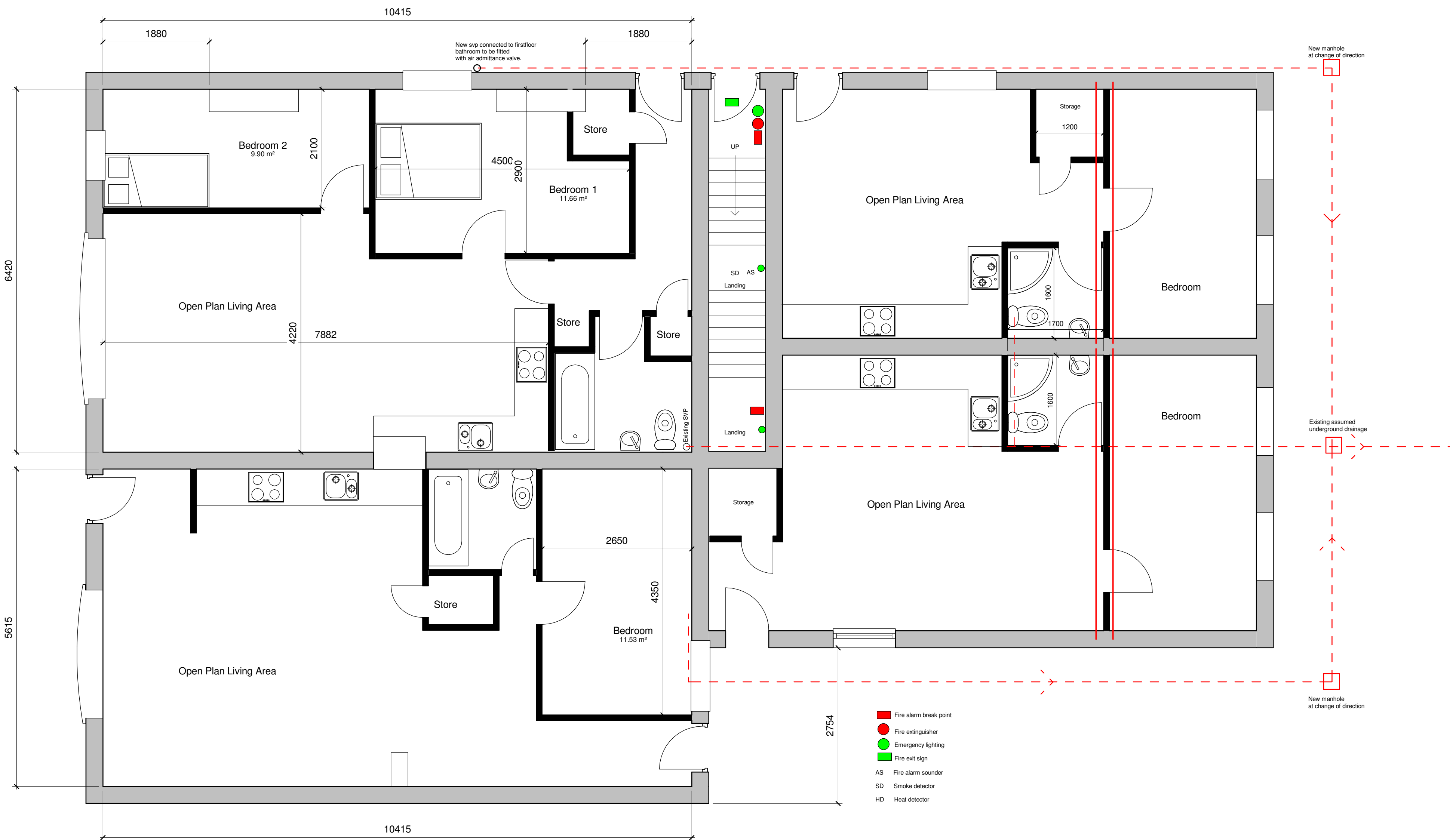
Proposed Ground Floor 1 : 50
