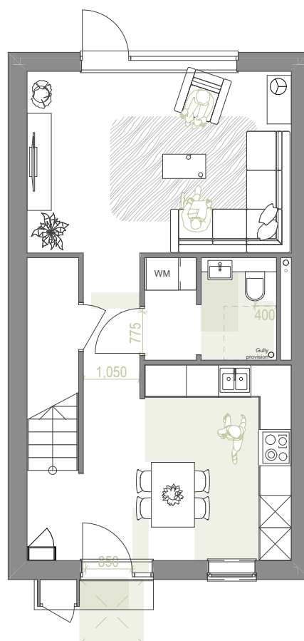
Ground Floor 1:100
