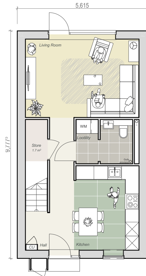
Ground Floor 1:100
