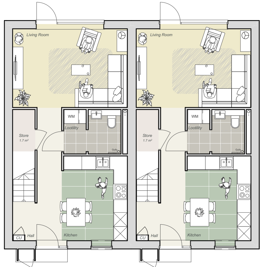
Ground Floor 1:100
