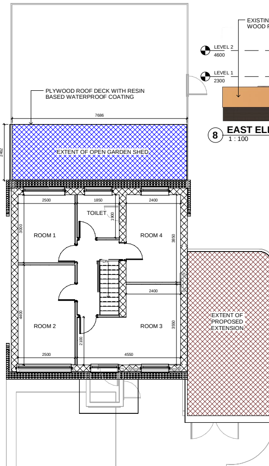
6 LEVEL 2 1:50
