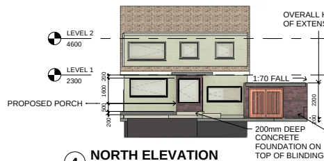
4 NORTH ELEVATION 1:100
