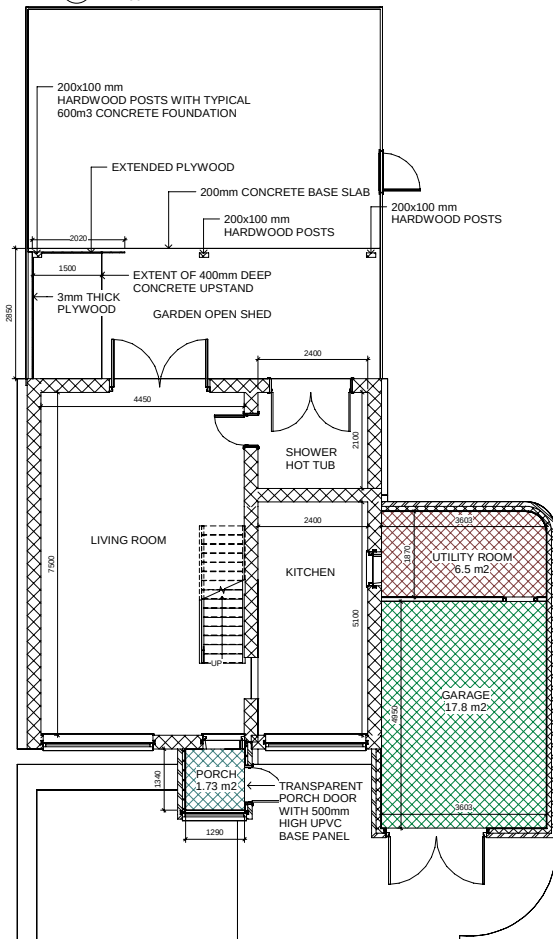
2 LEVEL 1 1:50
