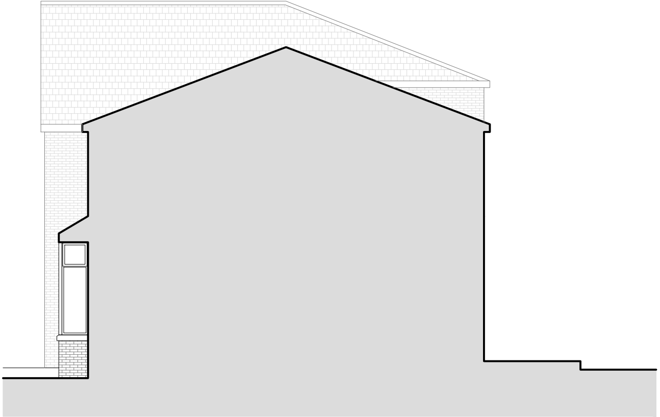
EXISTING SIDE ELEVATION 1:100 @ A2
