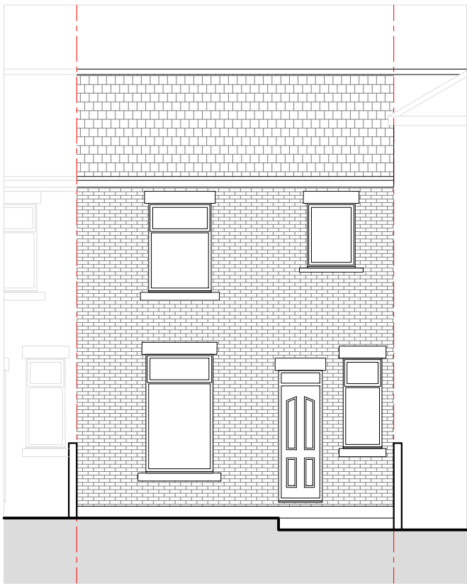
EXISTING REAR ELEVATION 1:100 @ A2
