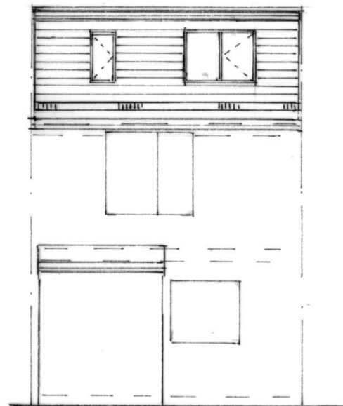
REAR ELEVATION (PROPOSED)
