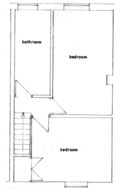
F.F PLAN (EXISTING)
