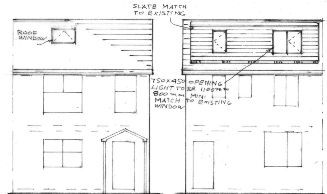
FRONT ELEVATION (PROPOSED)
