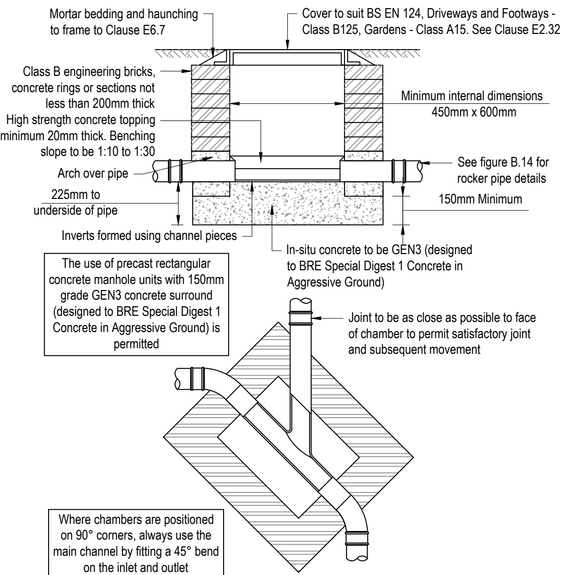
Typical Inspection Chamber Detail - Type 4 (Rigid material detail)
