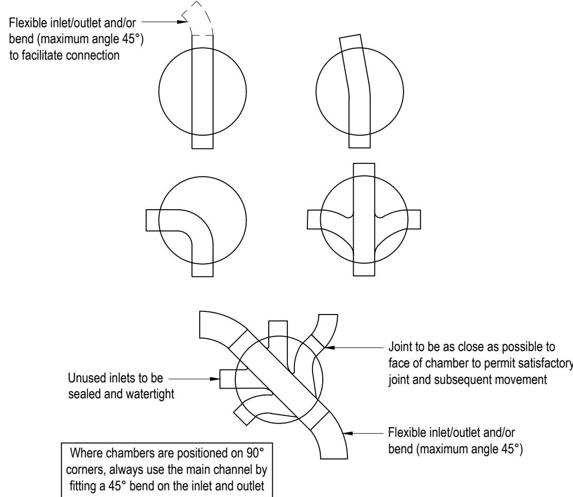
Alternative Base Layouts for Type 3 Chambers
