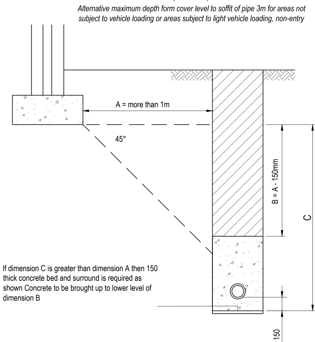
Drain trench edge more than 1m. from footing/foundation edge
