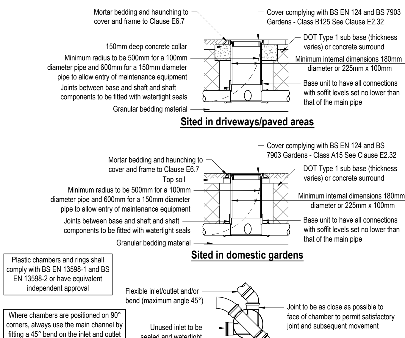
Typical Inspection Chamber Detail - Type 4 (Flexible Material Detail)
