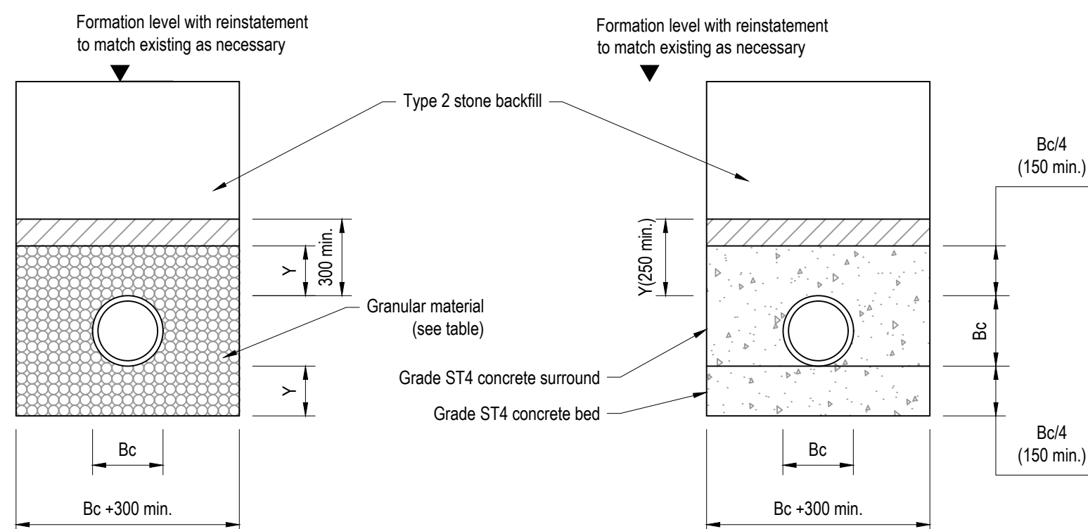
Class S Detail
