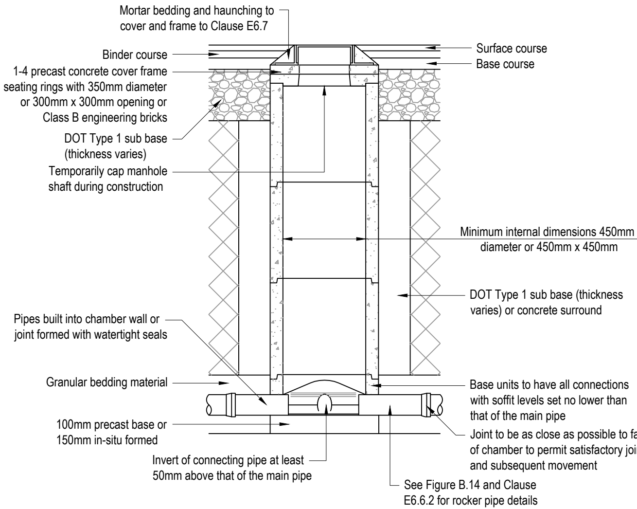
Typical Inspection Chamber Detail - Type 3 (Rigid Material Detail)
