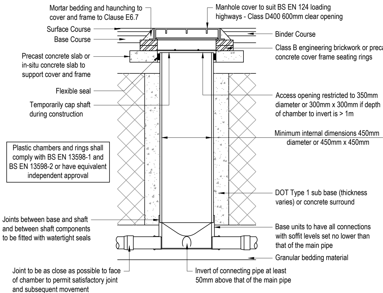
Typical Inspection Chamber Detail - Type 3 (Flexible Material Detail)
