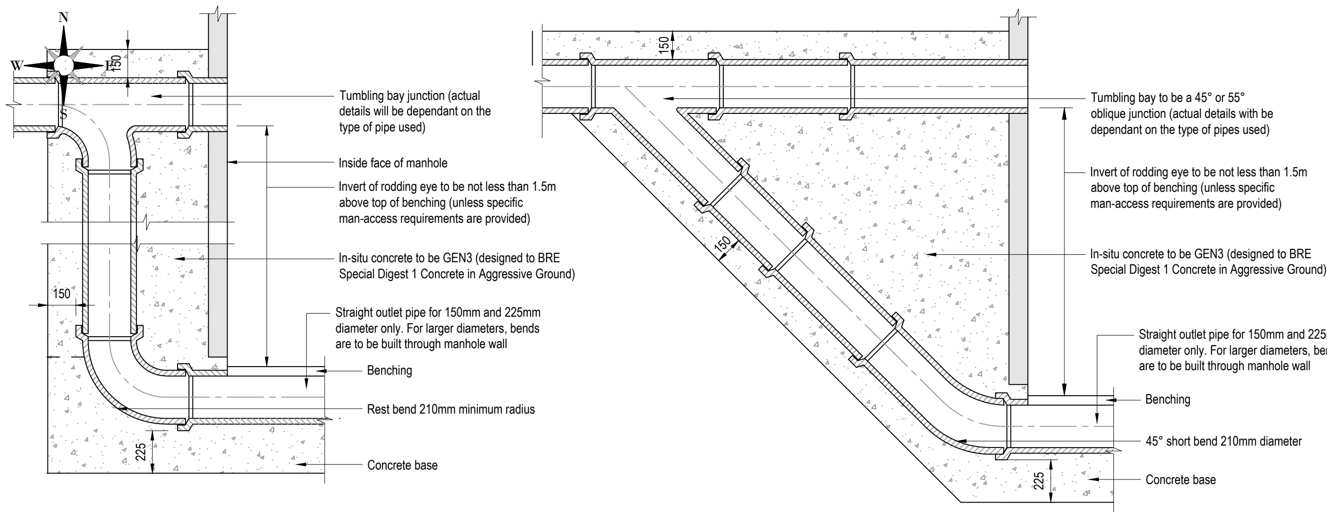
External Vertical Backdrop Detail
