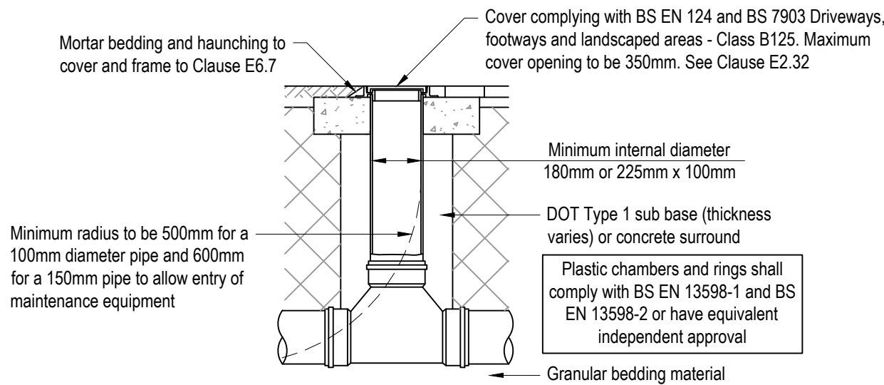
Typical Inspection Chamber Detail - Type 4 (Alternative Construction Detail)
