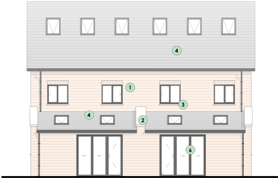
House Type A - Rear (NMA) 1 : 100
