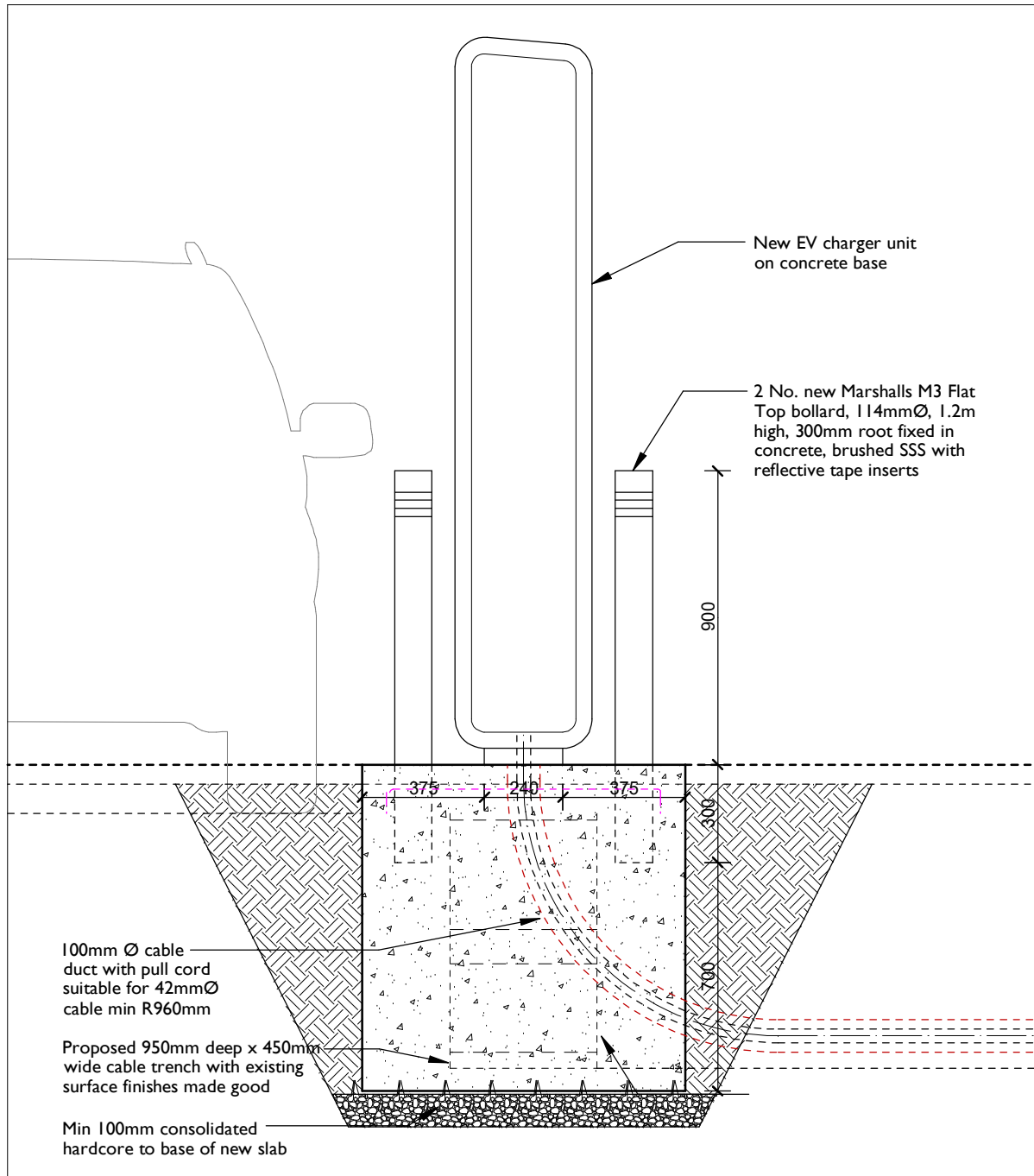
FRONT ELEVATION 1:20
