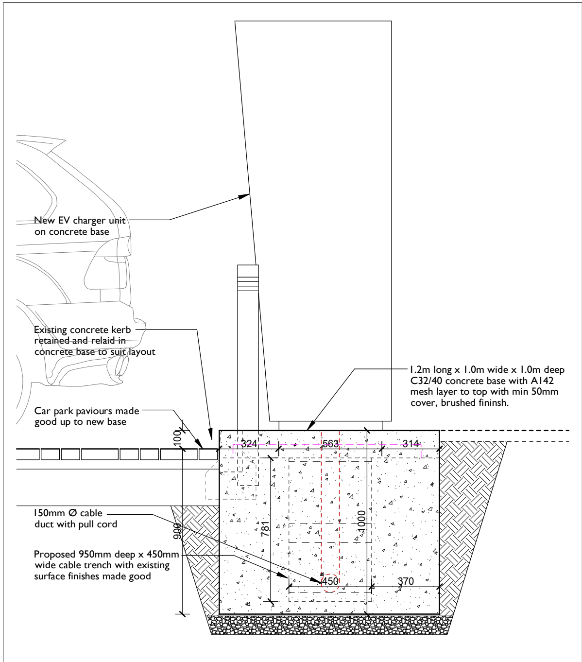
SECTION 1:20
