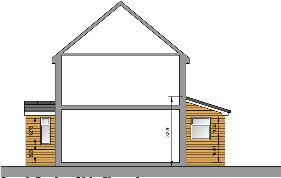
South Facing Side Elevation
