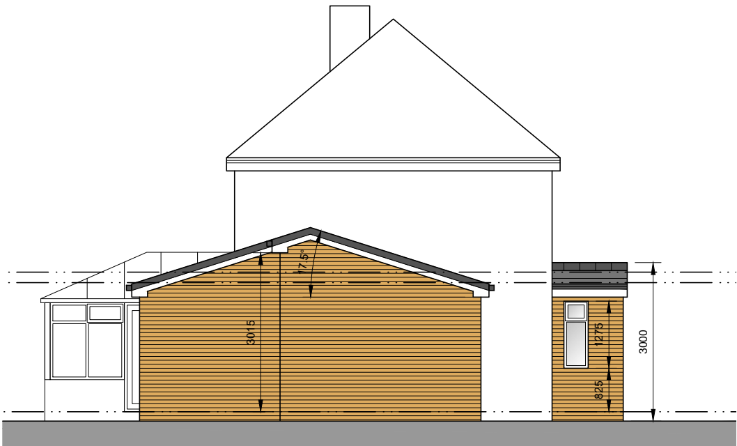
North Facing Side Elevation
