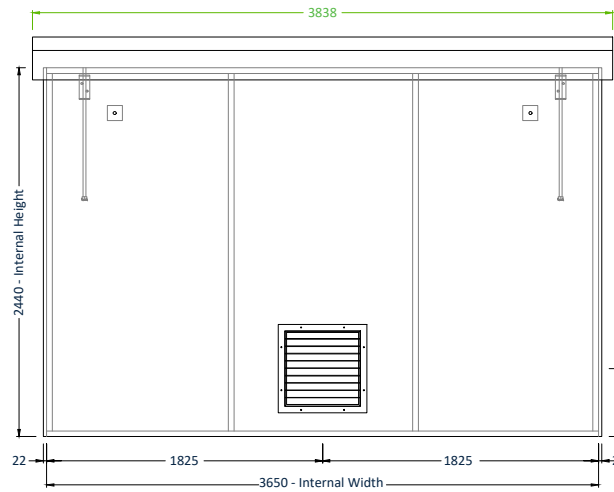
RH SIDE ELEVATION
