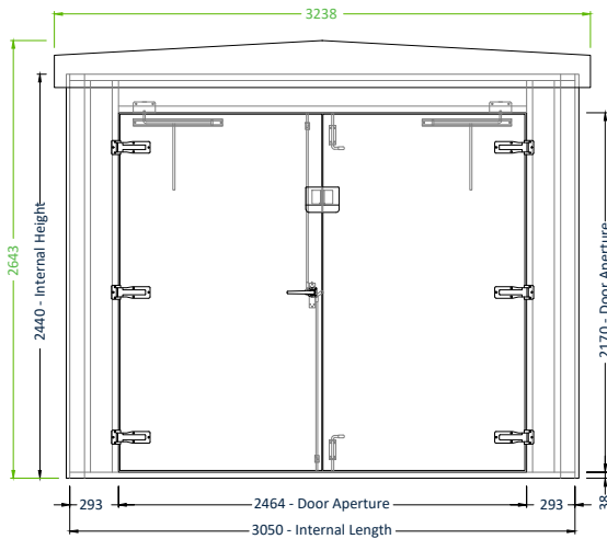
FRONT ELEVATION
