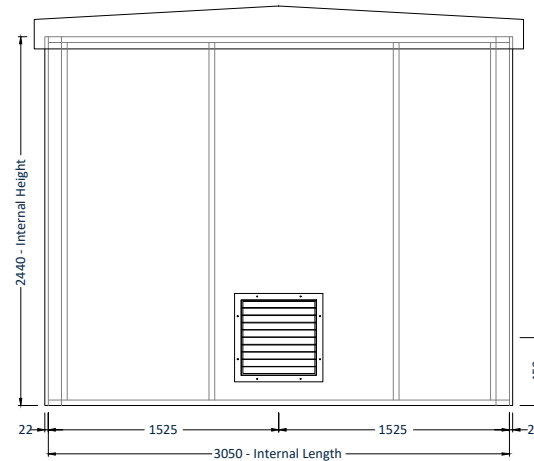
REAR ELEVATION
