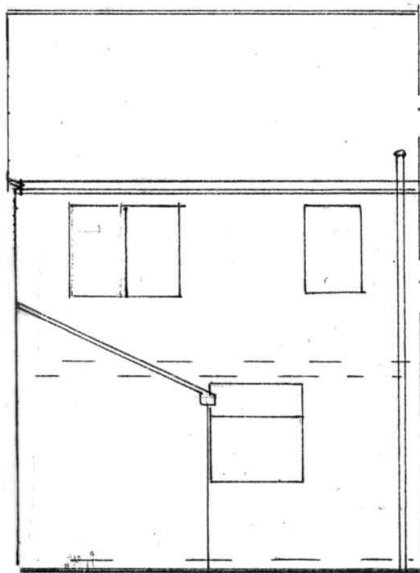
REAR ELEVATION (EXISTING)
