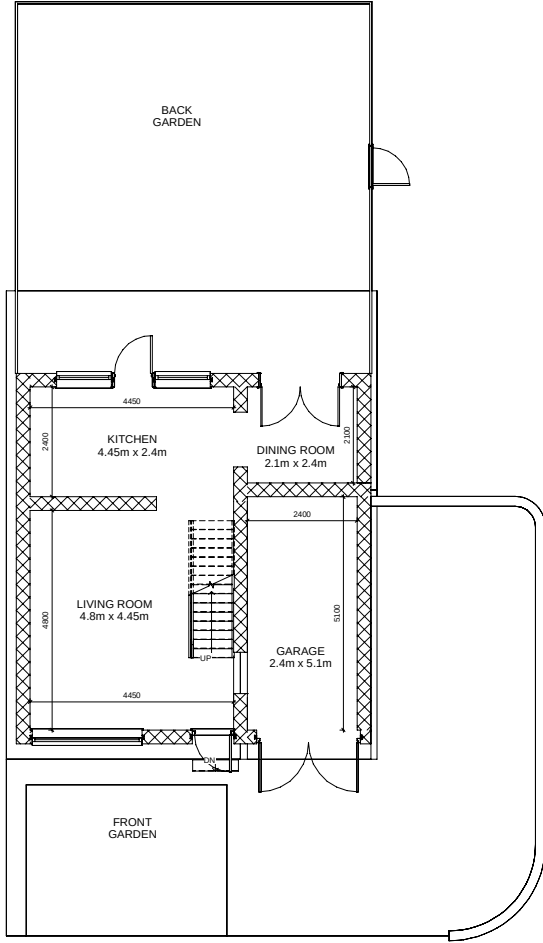
4 LEVEL 1 1:50
