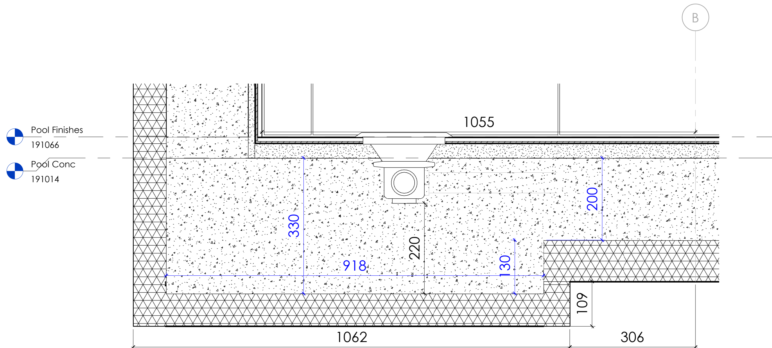
2 Main Drain Detail 1 : 5
