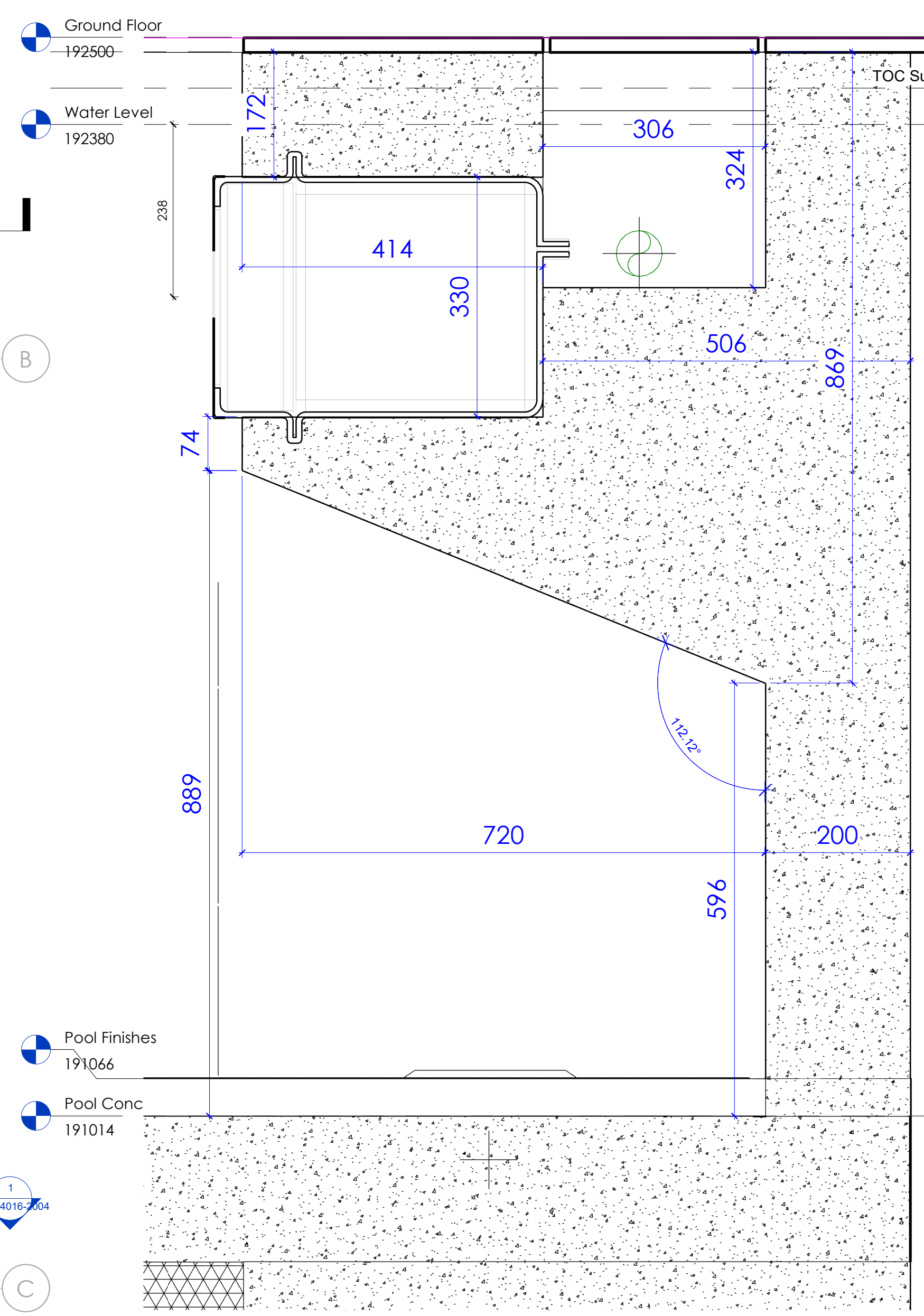
2 Eva Detail - Concrete 1 : 5
