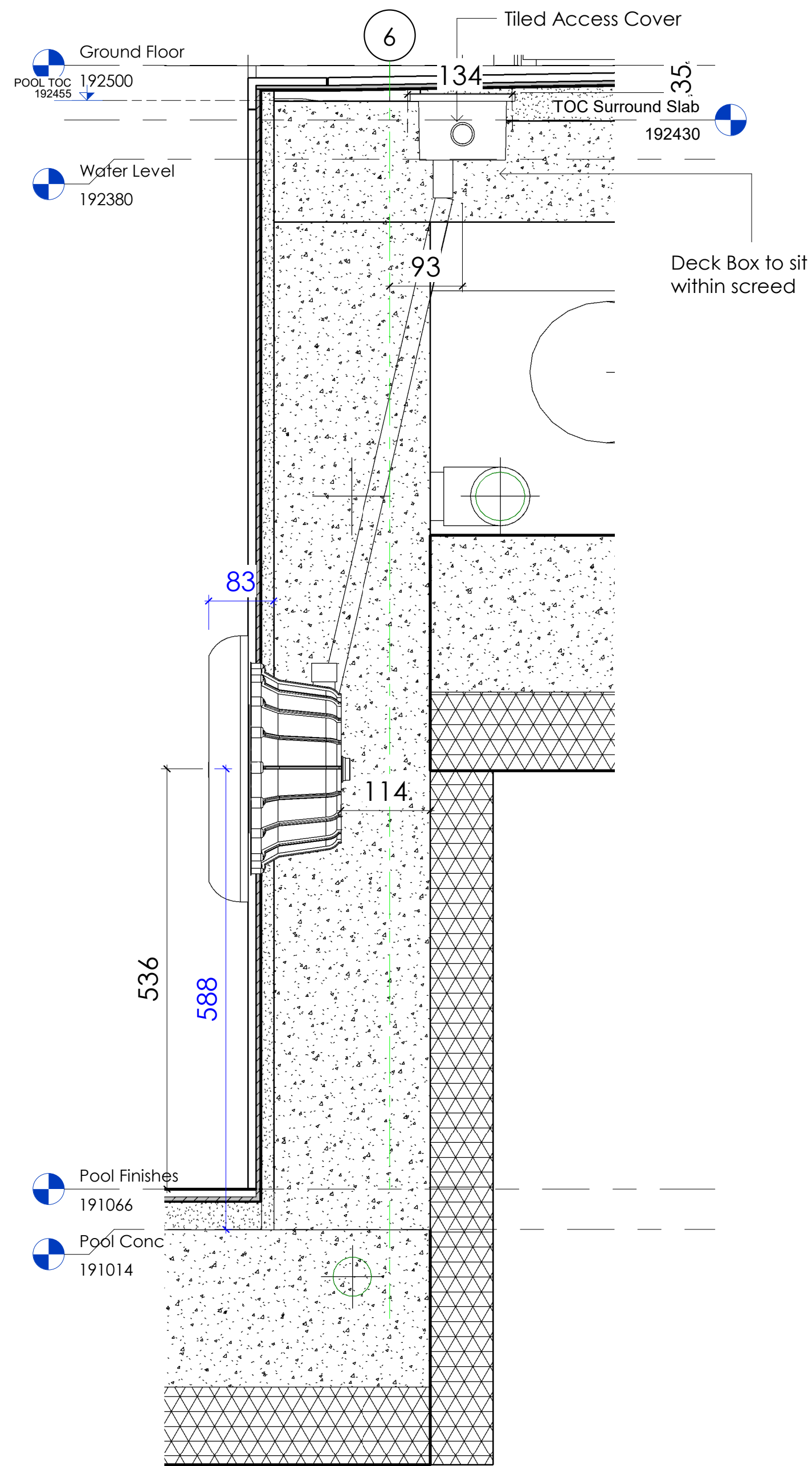
3 Skimmer Detail 1 : 5
