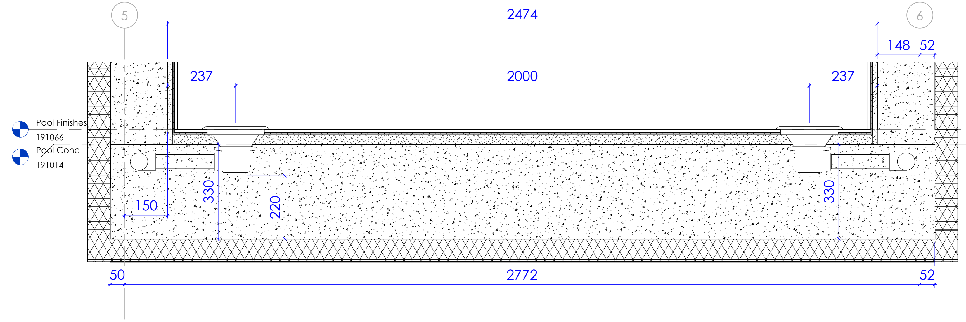
5 Concrete drain section 1 : 7
