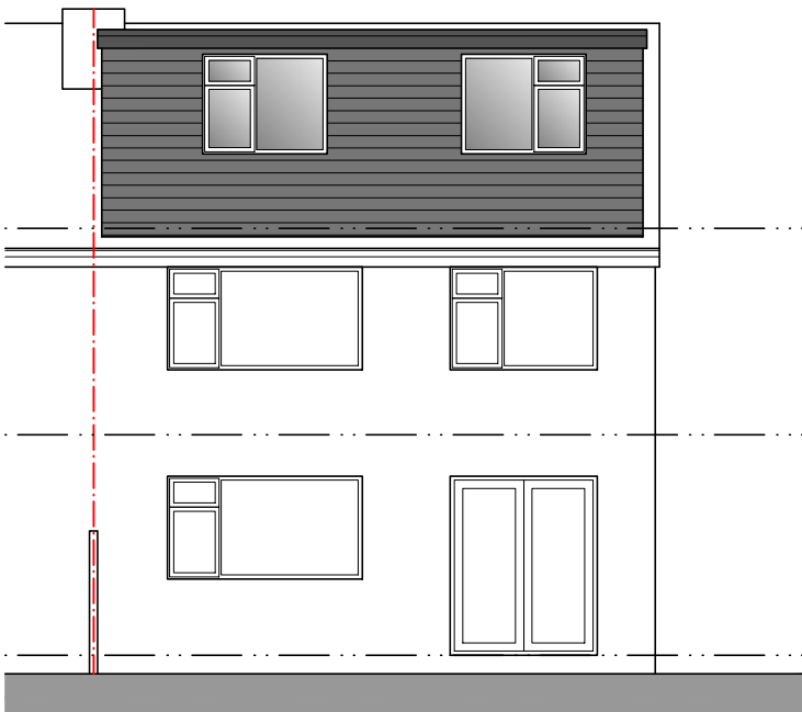
South East Facing Rear Elevation
