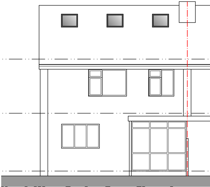
North West Facing Front Elevation
