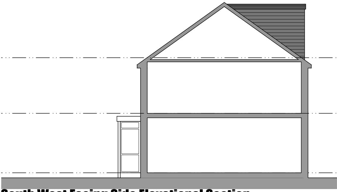
South West Facing Side Elevational Section
