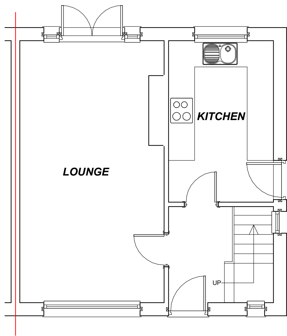
Existing Ground Floor Layout 1 : 50
