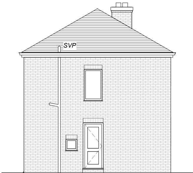
Existing Side Elevation A (View From No.16) 1 : 100
