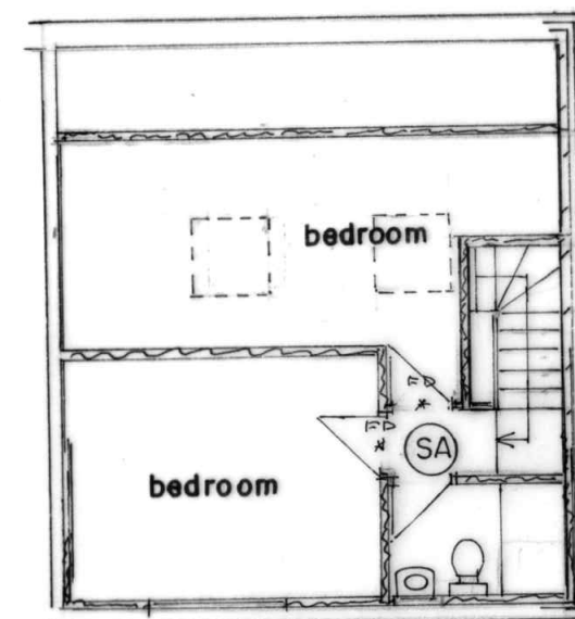
SECOND FLOOR PLAN (PROPOSED)
