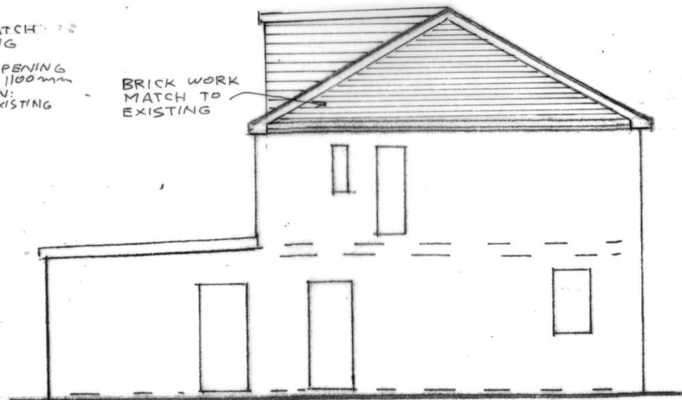
SIDE ELEVATION (PROPOSED)
