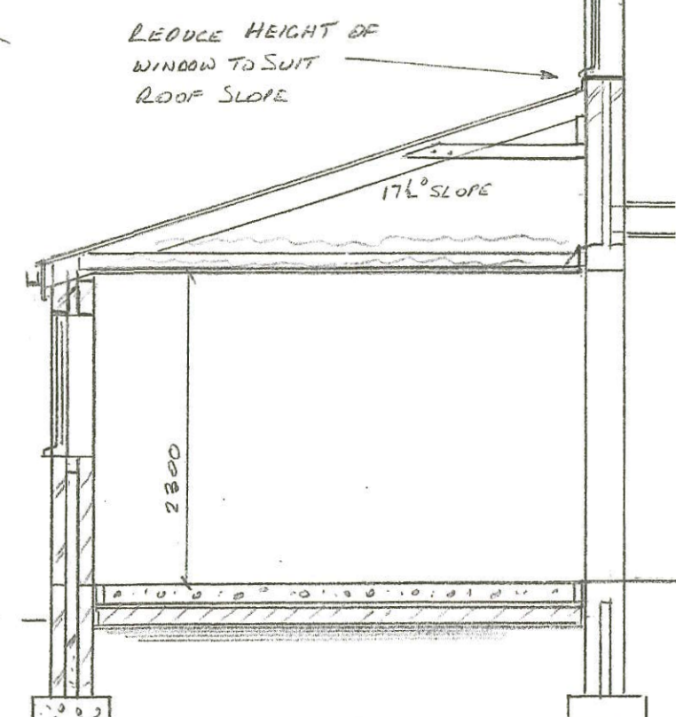
PROPOSED SIDE ELEVATION FROM N°31
