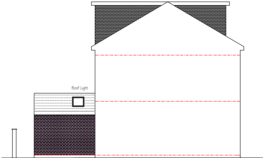
Elevation From No 10
