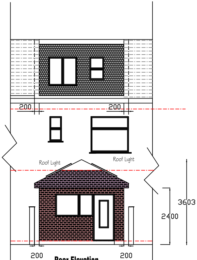
Rear Elevation
