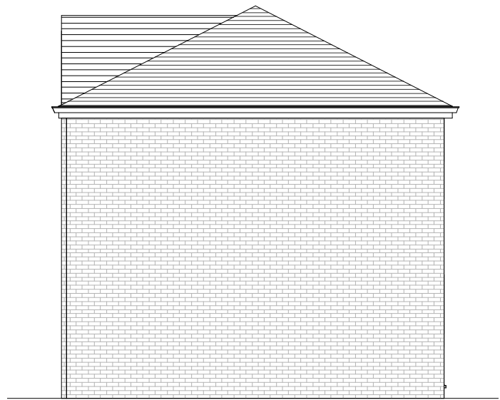
Existing Side Elevation A (View From No.60) 1 : 100
