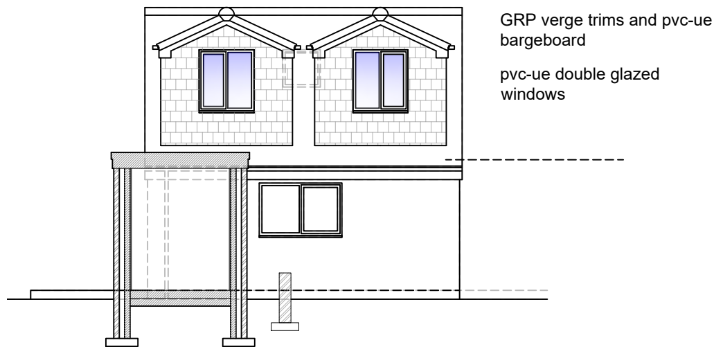
PROPOSED ELEVATION DD scale 1 - 100
