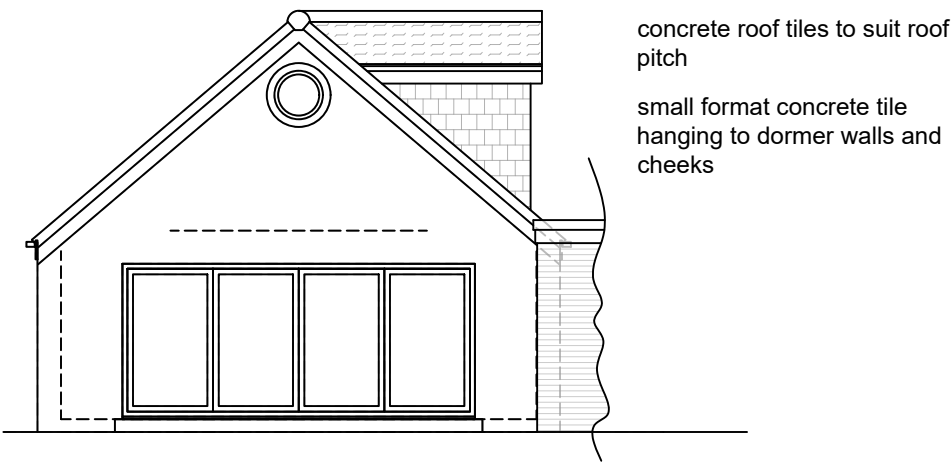
PROPOSED ELEVATION EE scale 1 - 100
