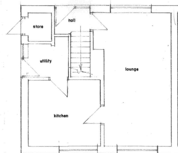
G.F. PLAN (EXISTING)
