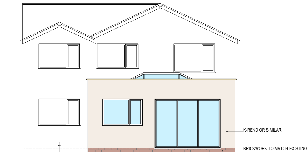
PROPOSED REAR
