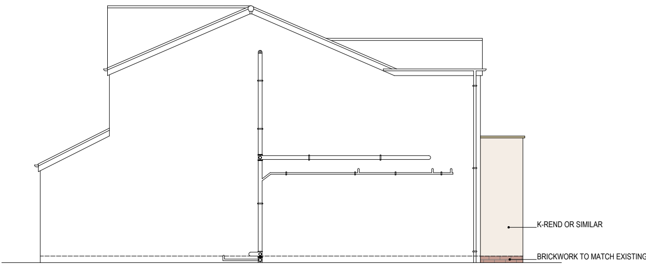
PROPOSED SIDE
