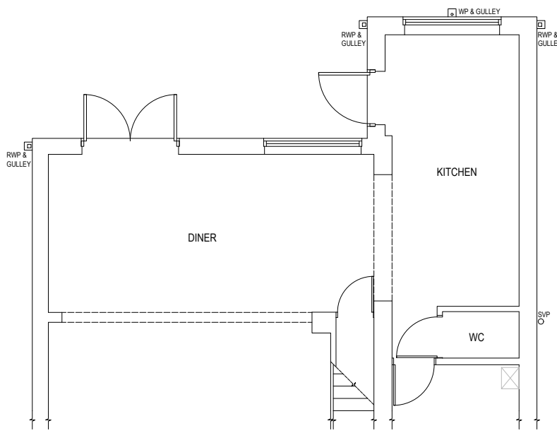
EXISTING GROUND
