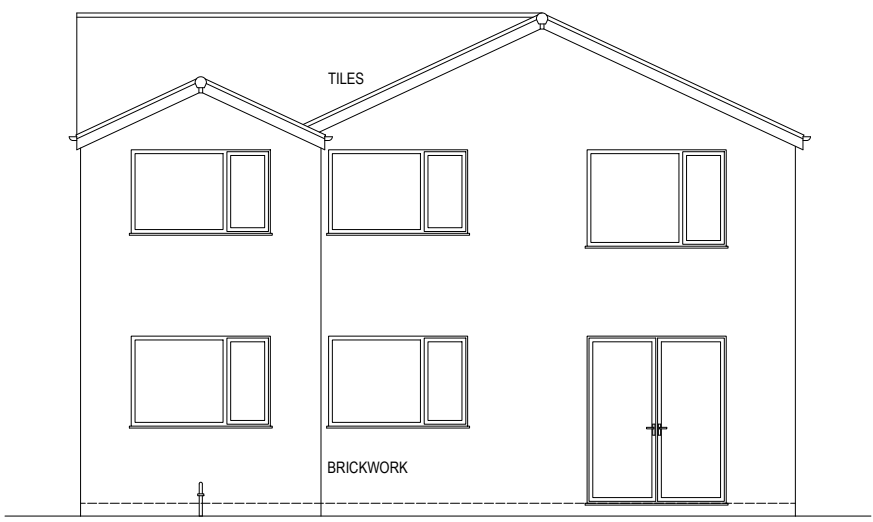
EXISTING REAR
