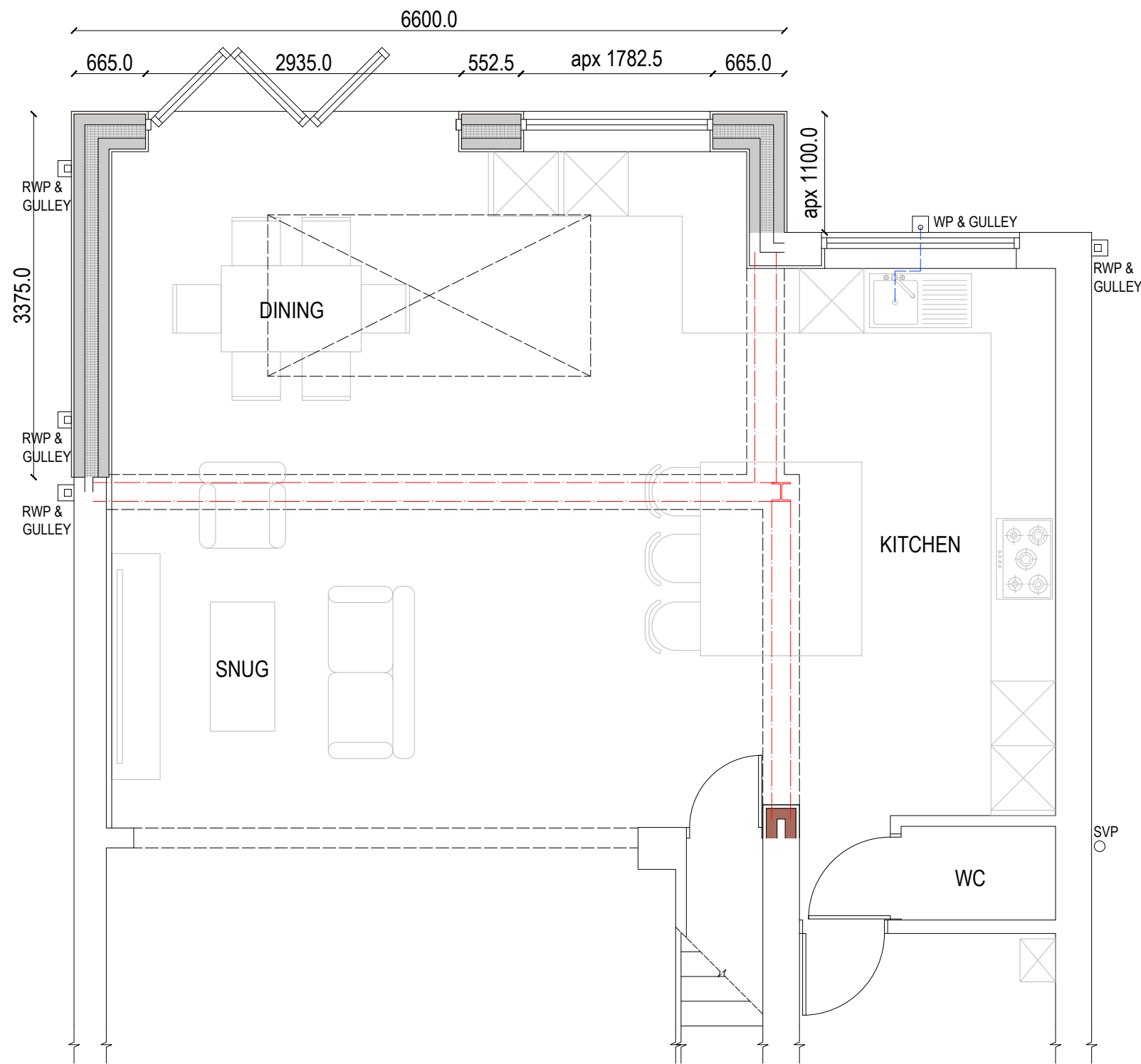
PROPOSED GROUND
