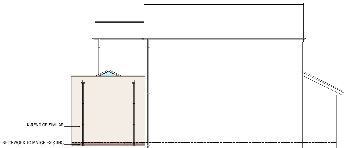
PROPOSED SIDE
