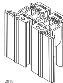
2810 Horizontal Mech Joint (pair)
