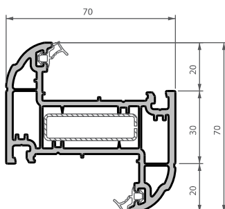
2836 Z transom/mullion
