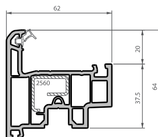
2802 flush window sash
