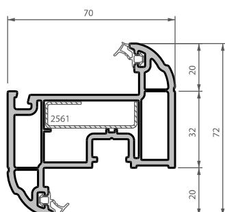
2826 externally beaded casement sash
