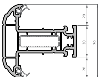
2835 T transom/mullion
