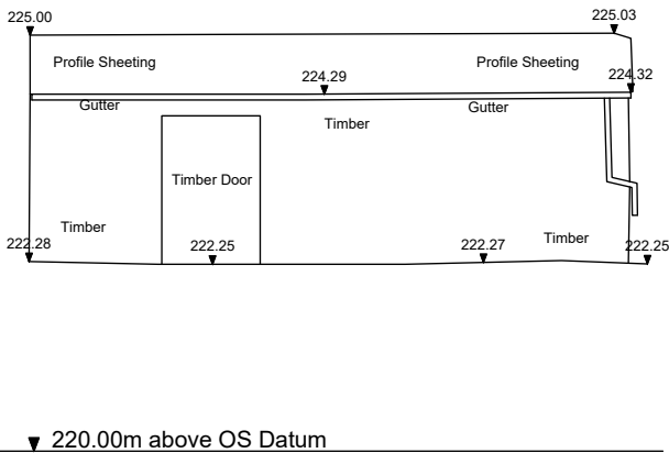
Existing B3 East Elevation
