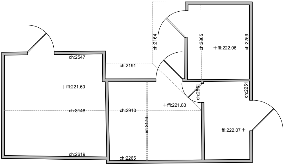
Existing B3 Ground Floor Plan
