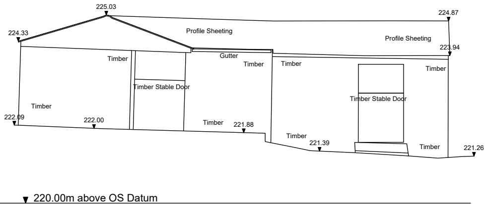
Existing B3 North Elevation
