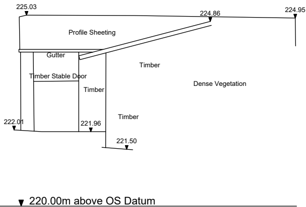
Existing B3 West Elevation
