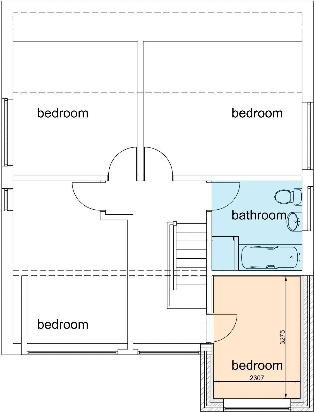
PROPOSED FIRST FLOOR - OPTION 1 scale 1 - 50
