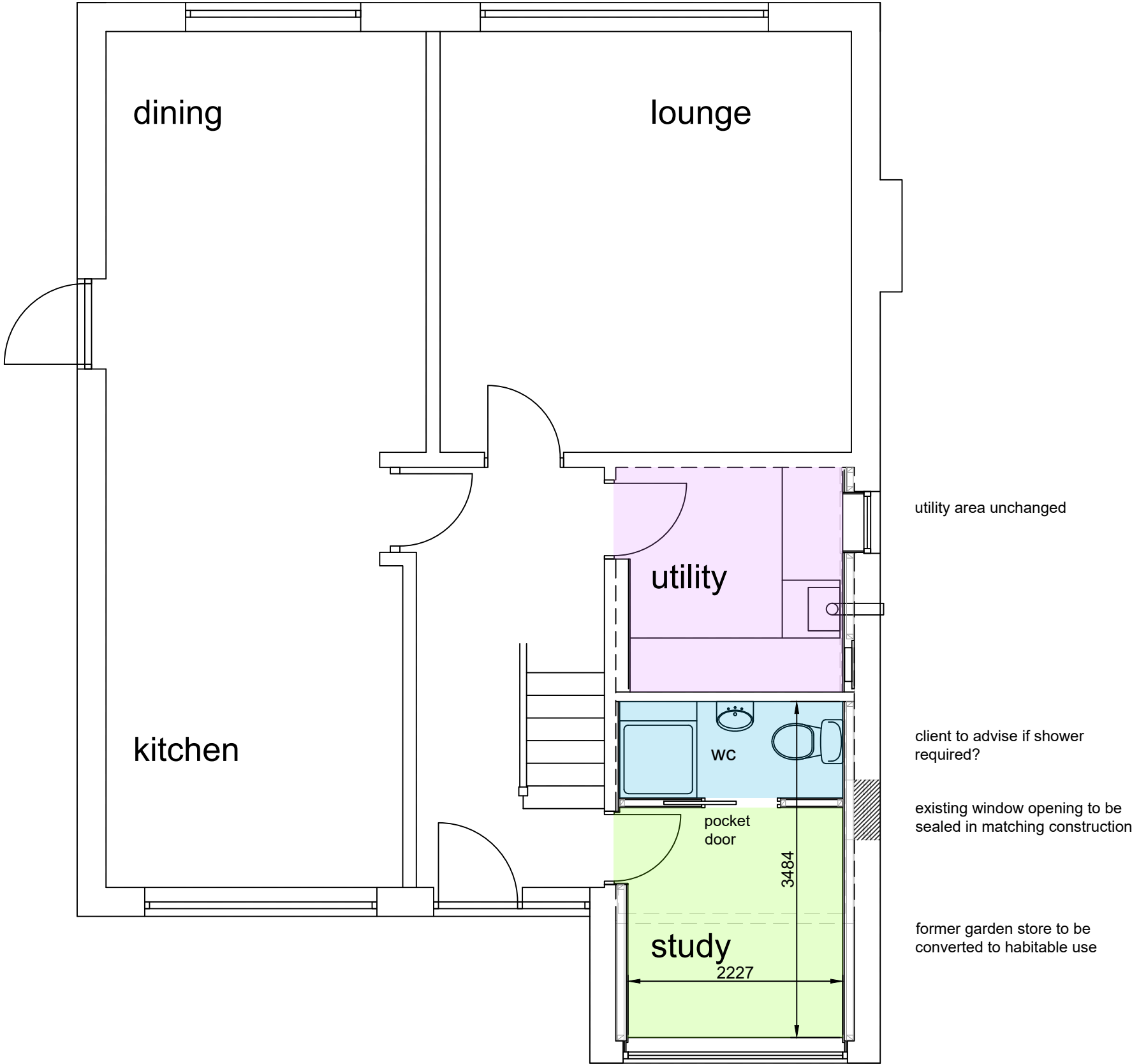
PROPOSED GROUND FLOOR - OPTION 1 scale 1 - 50
