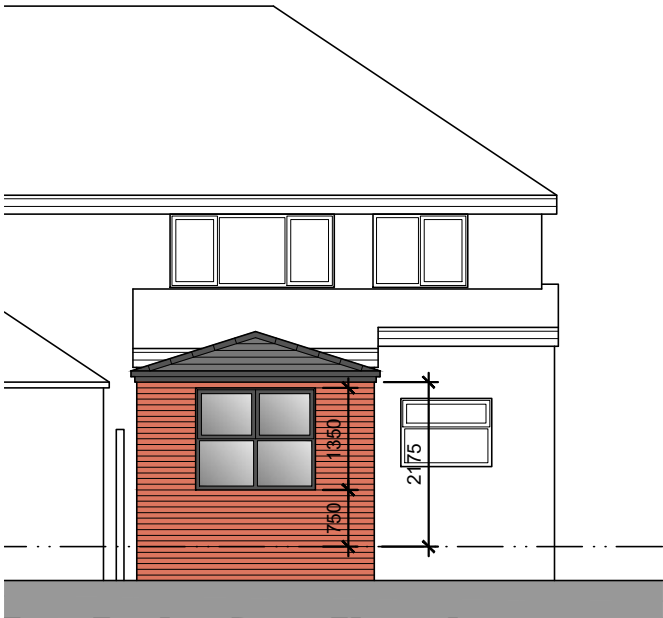
East Facing Rear Elevation
