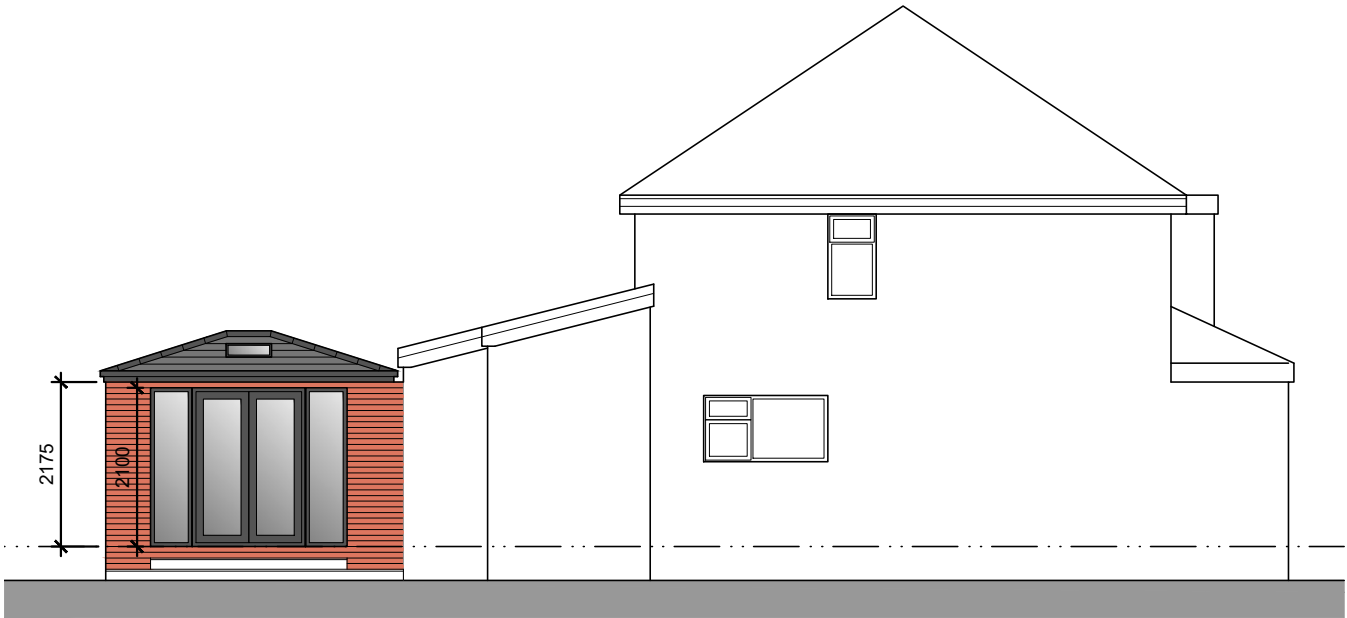
North Facing Side Elevation
