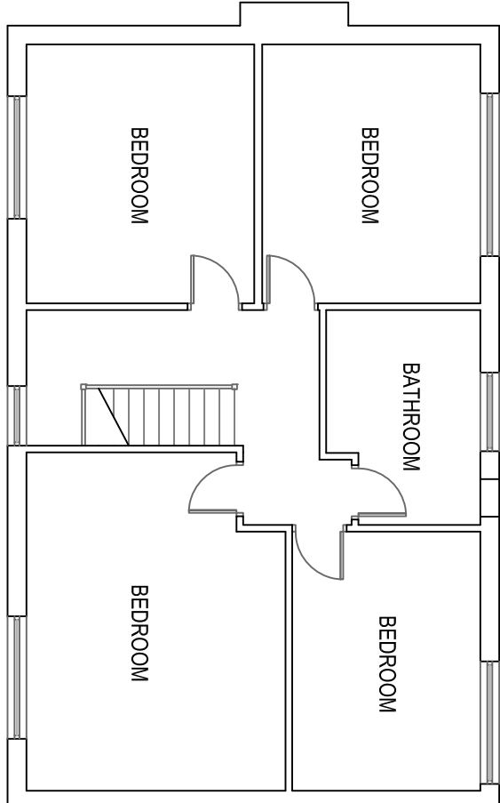
PROPOSED FF PLAN 1:100
