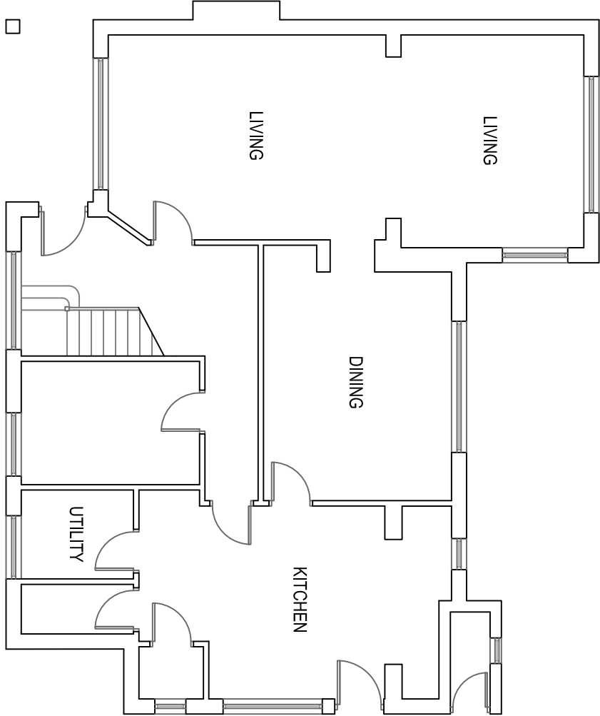
EXISTING GF PLAN 1:100
