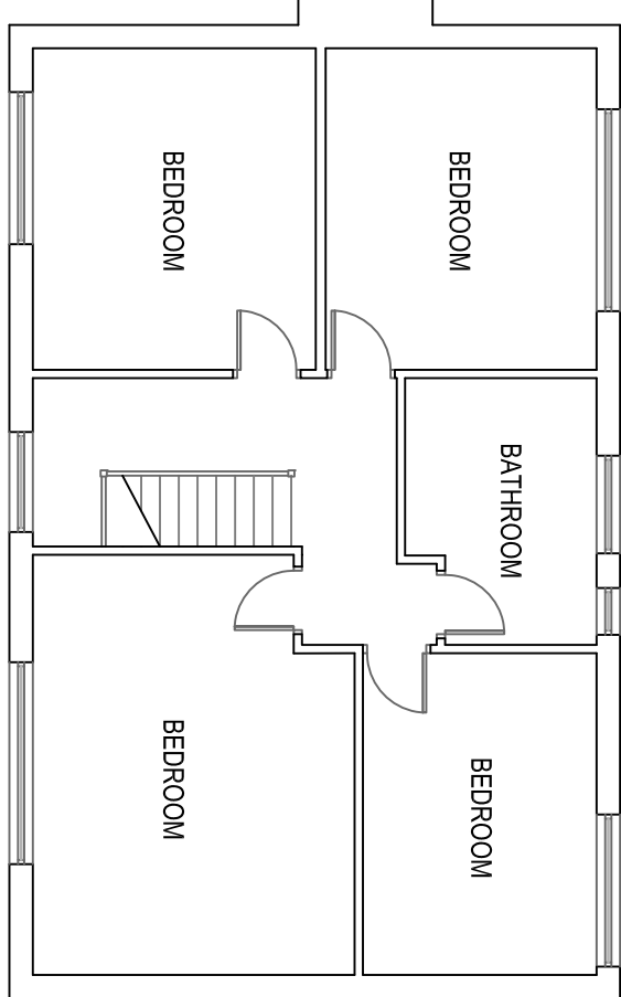
EXISTING FF PLAN 1:100
