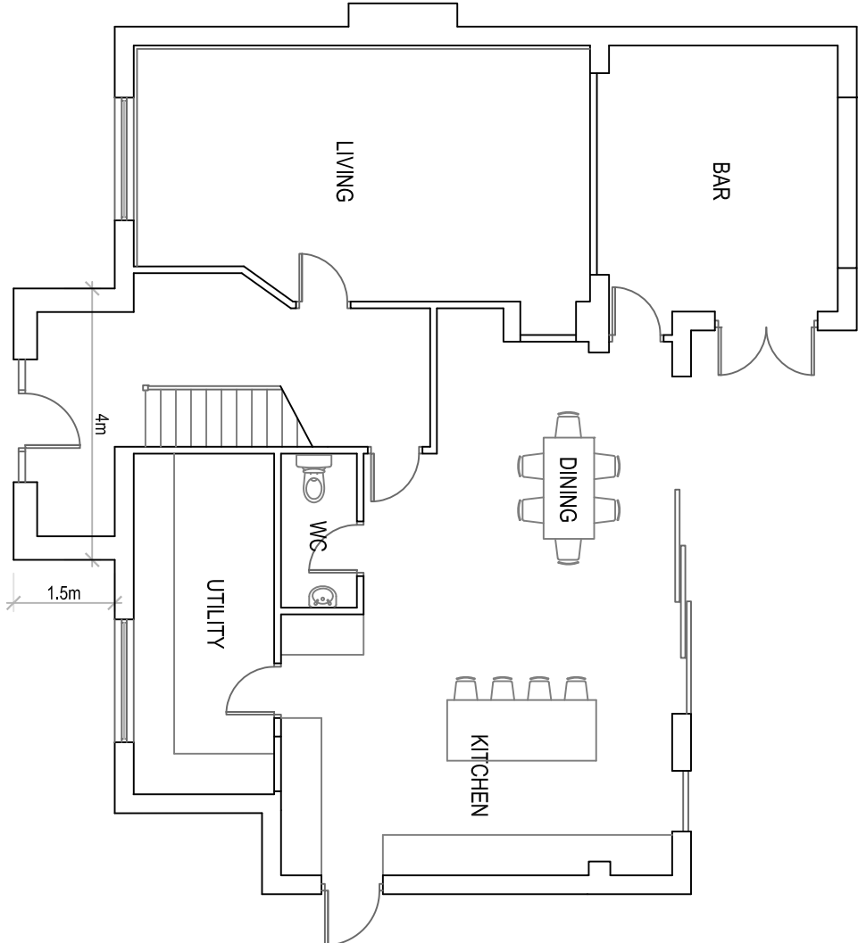
PROPOSED GF PLAN 1:100
