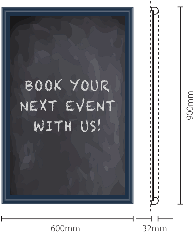
Scale : 1:10 @ A3 Item F1. 1no. Powder coated aluminium chalkboard sign. G/CI - 800mm D - 32mm
