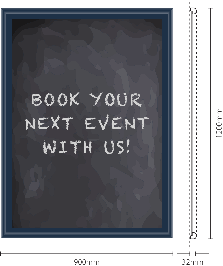
Scale : 1:10 @ A3 Item F2. 1no. Powder coated aluminium chalkboard sign. G/CI - 1280mm D - 32mm
