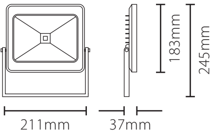
Scale : 1:10 @ A3 Item I. 7no. Floodlights. (see CSI 233 L for details) G/CI - 4360mm D - 245mm
