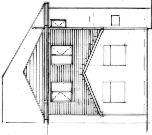
REAR ELEVATION (PROPOSED)
