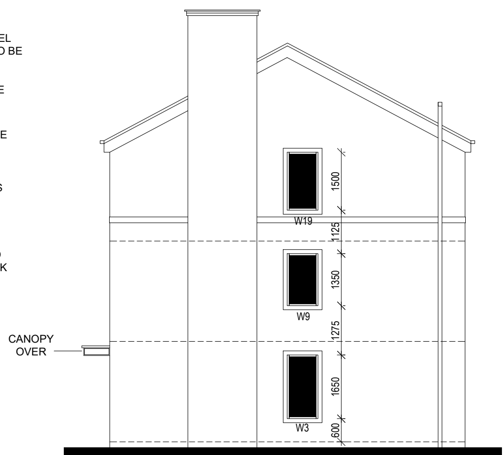
SIDE ELEVATION
