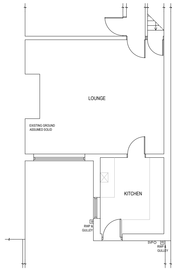
EXISTING GROUND
