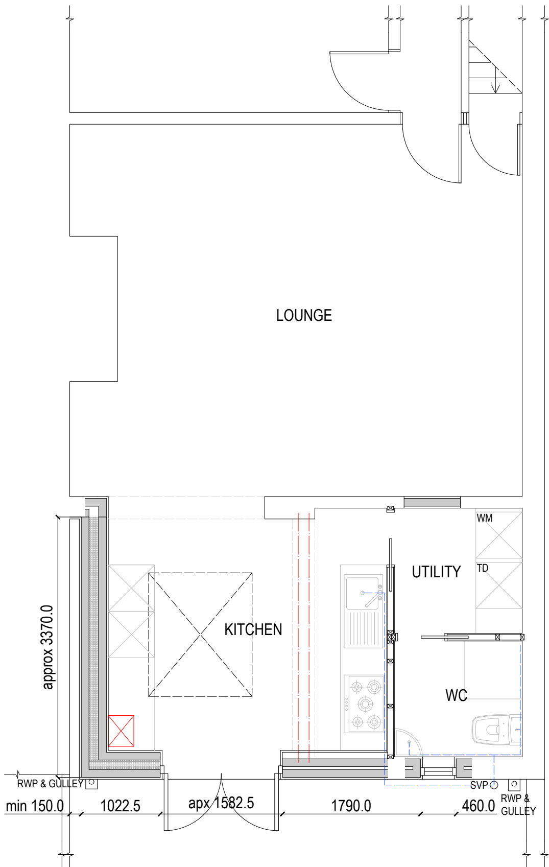
PROPOSED GROUND
