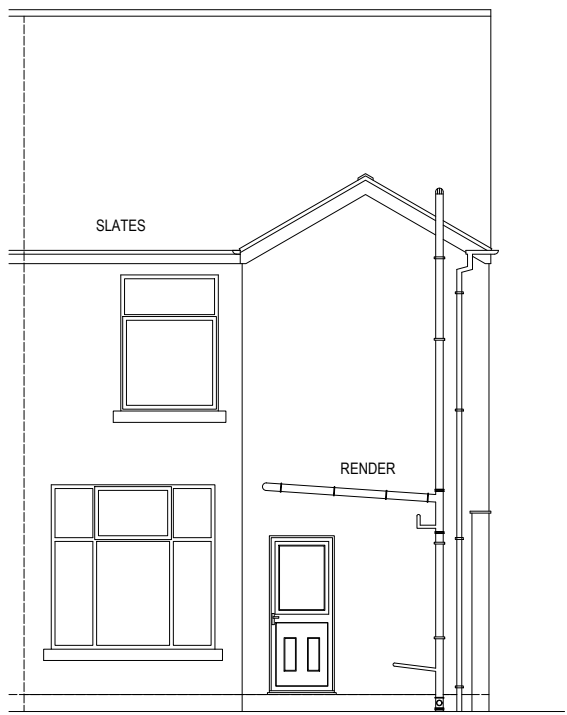
EXISTING REAR
