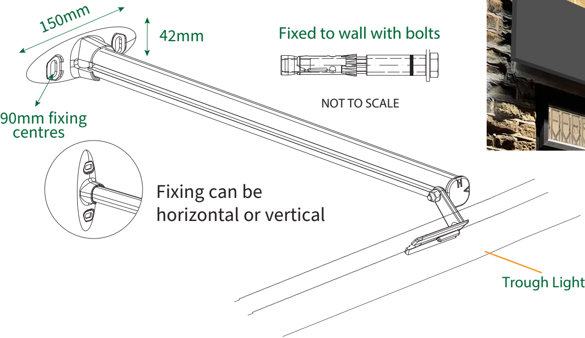
Trough light fixing for Item A.
