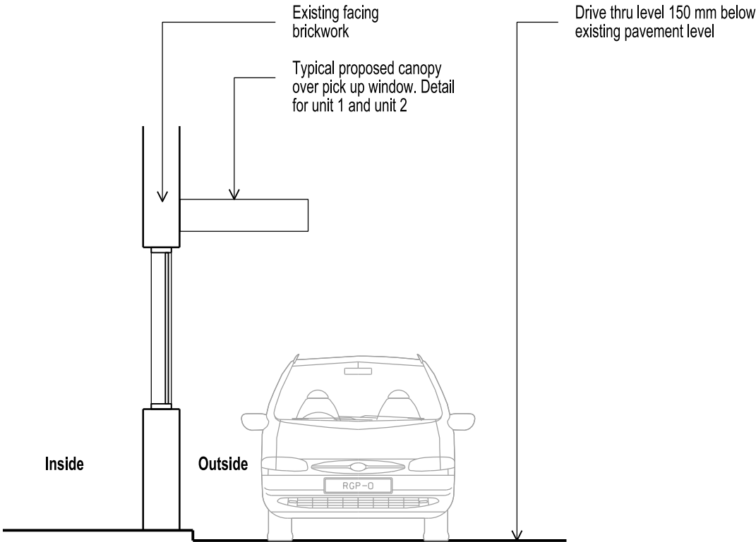
PROPOSED TYPICAL SECTION DETAIL
