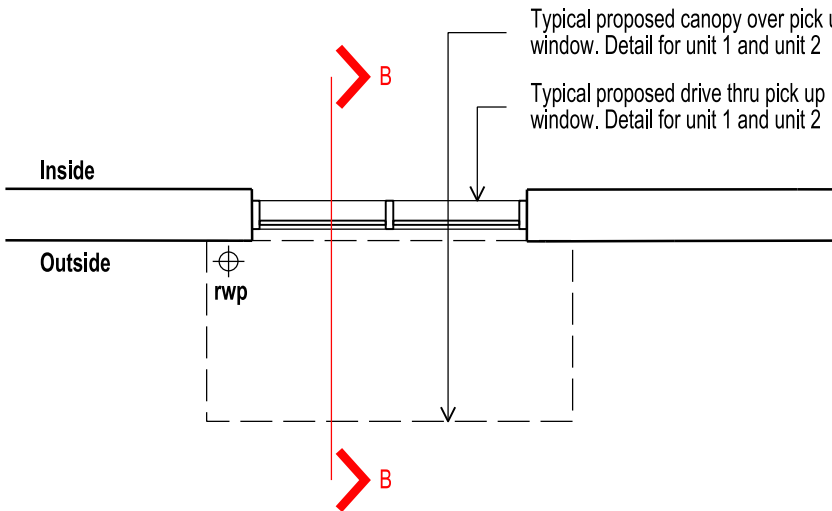
PROPOSED TYPICAL PLAN DETAIL
