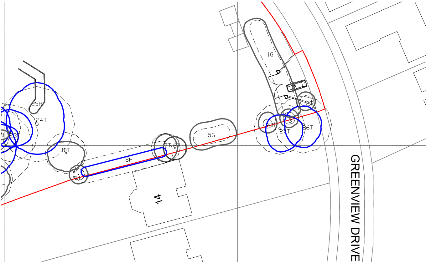
PROPOSED SITE PLAN 1:500
