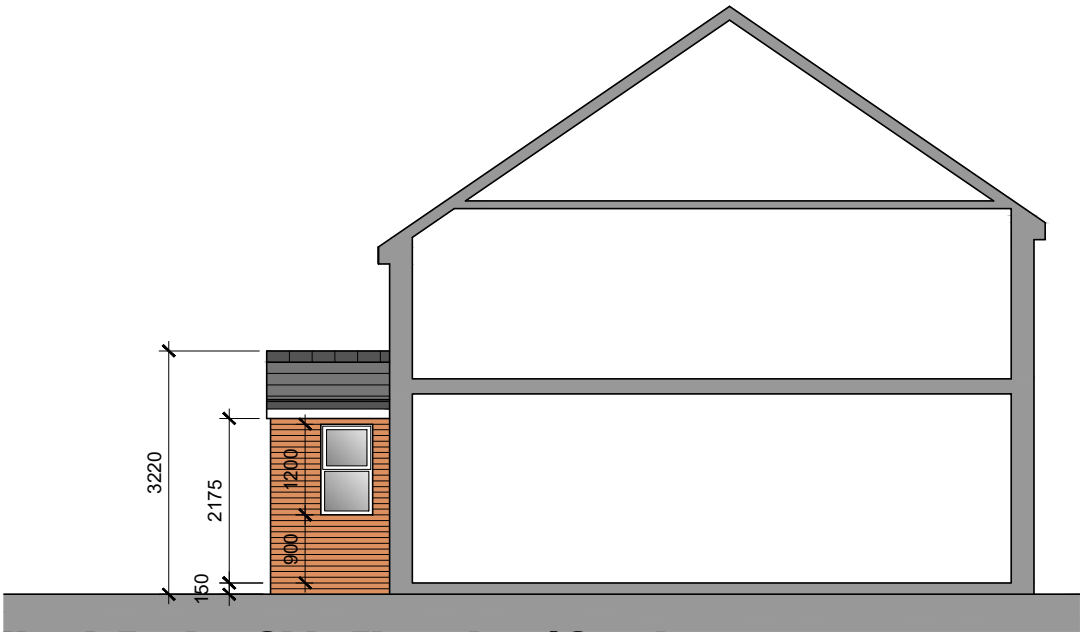
North Facing Side Elevation / Section
