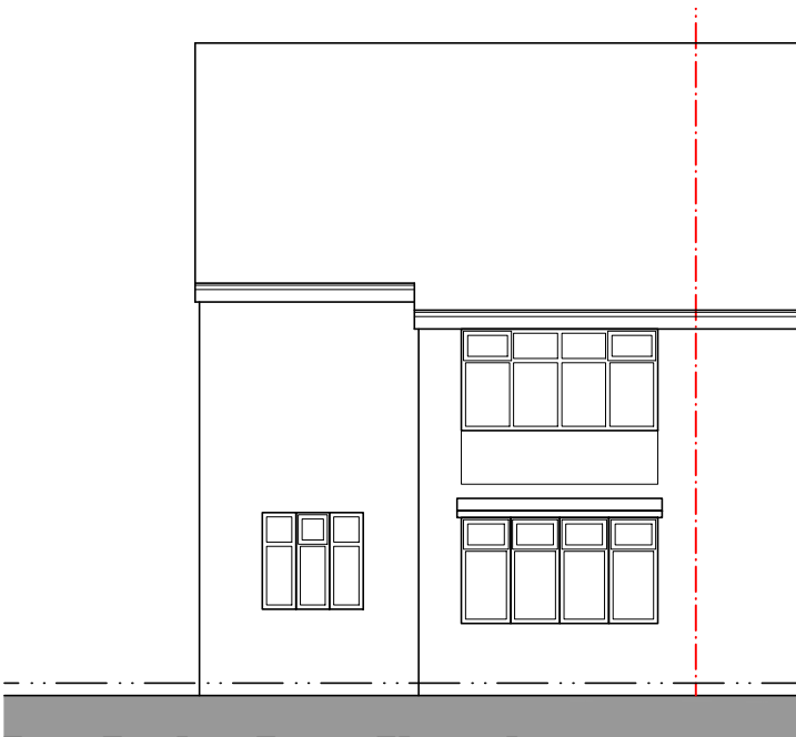
East Facing Front Elevation
