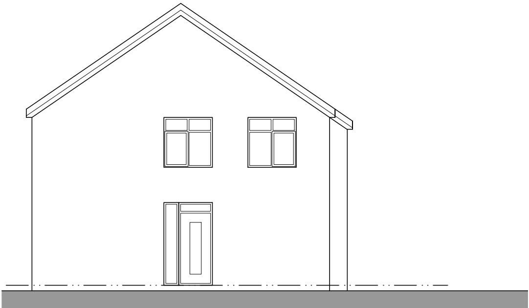
South Facing Side Elevation
