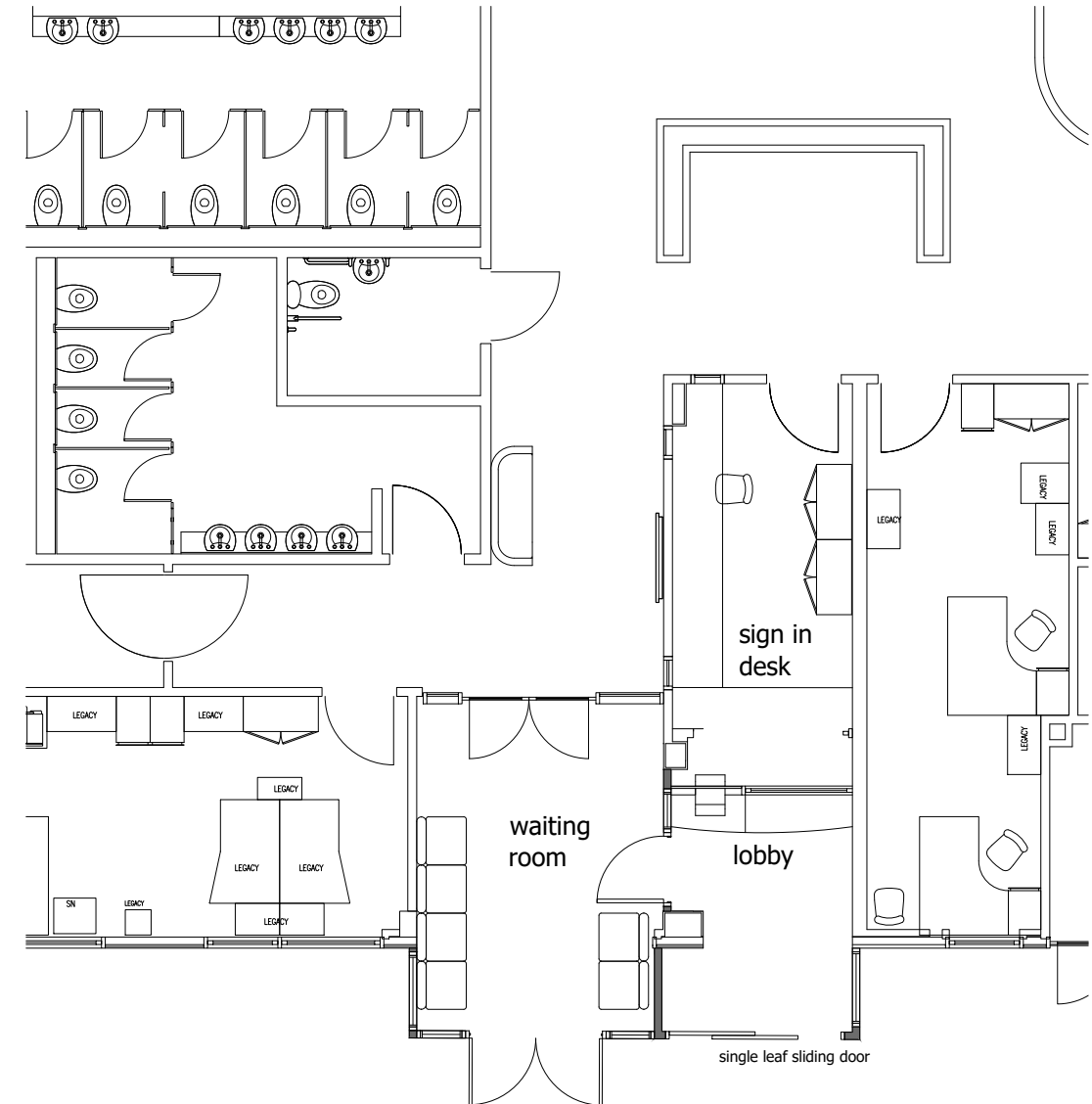
○ new doors (kept locked for security) linked to fire alarm system ○ ground floor plan as proposed
