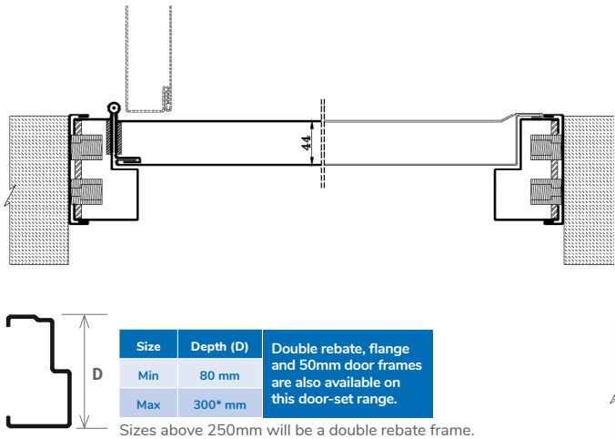
Fig.1 Single door with single rebate frame assembly
