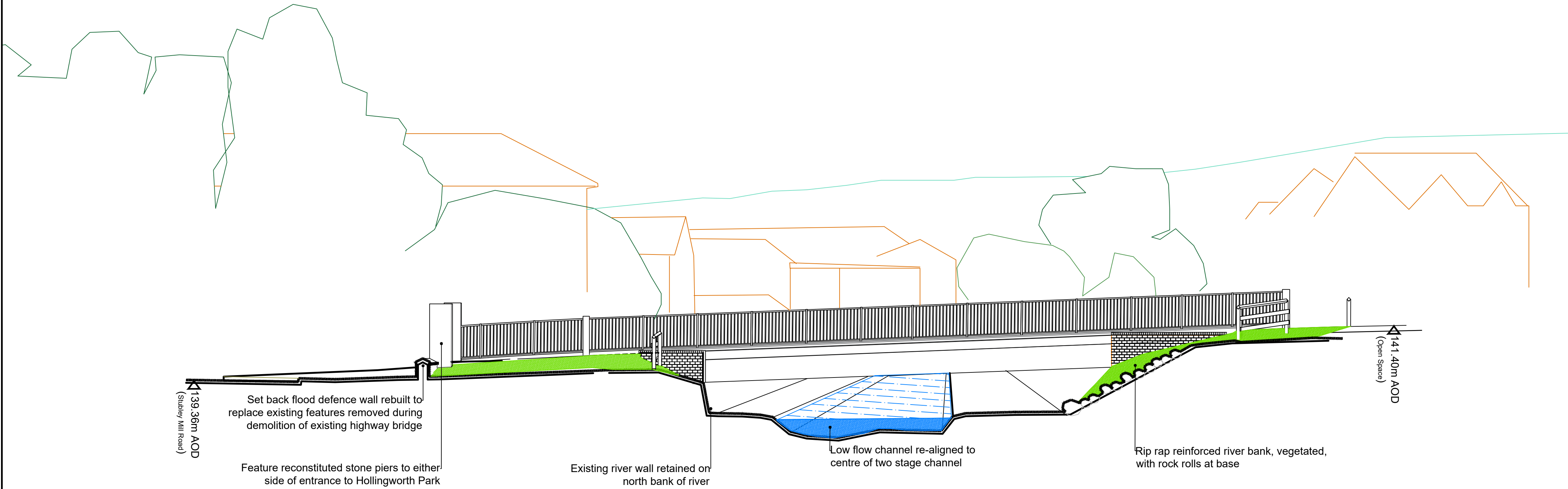
Elevation B - Riverstone Bridge Elevation view looking upstream Scale 1:100 @ A1
