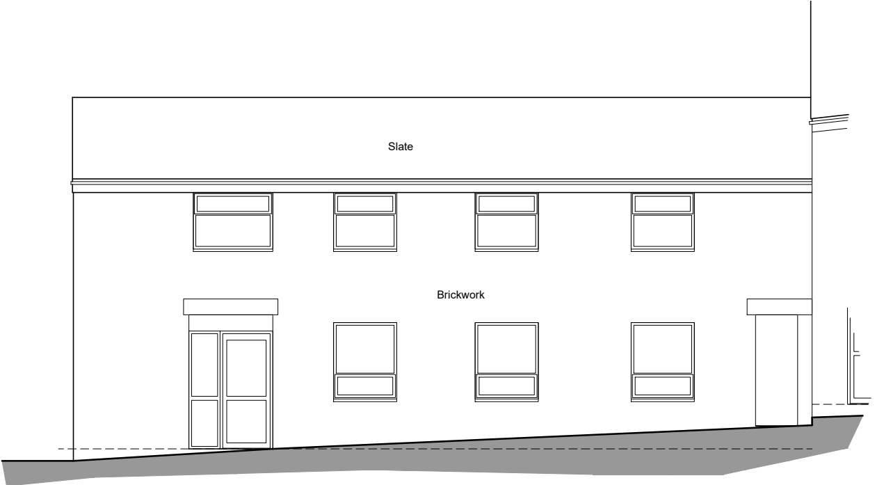
Rear Elevation
