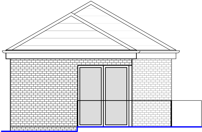
OUTBUILDING A PROPOSED SIDE ELEVATION
