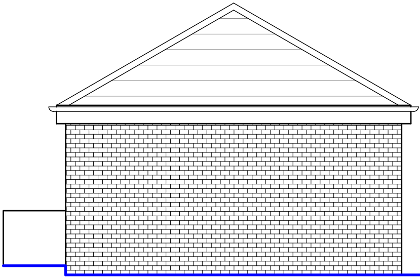
OUTBUILDING A PROPOSED SIDE ELEVATION
