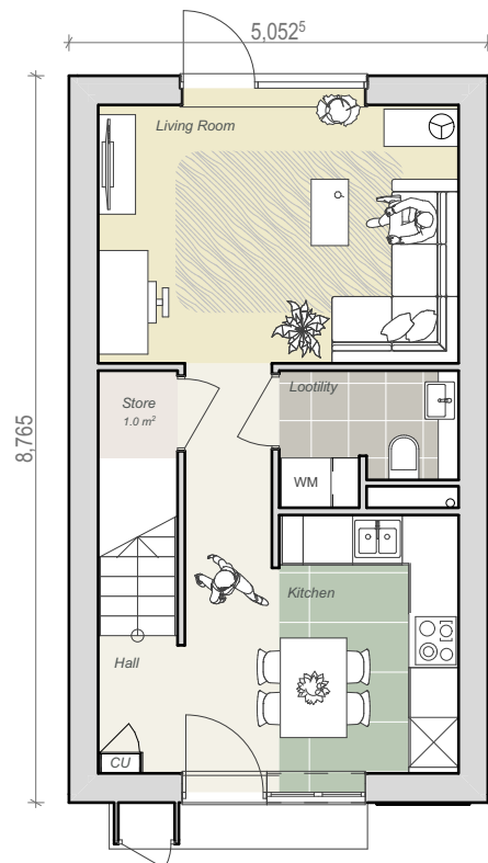
Ground Floor 1:100
