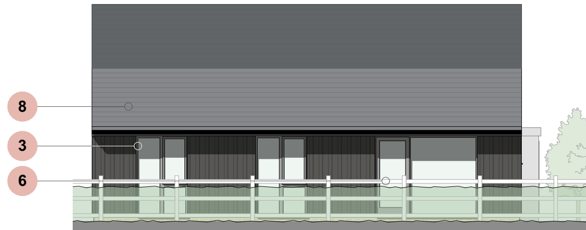
Side 1 Elevation 1:100
