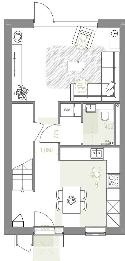
Ground Floor 1:100
